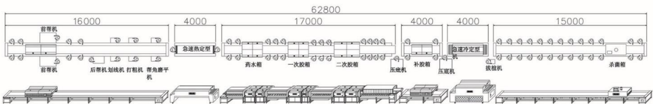
标准电路控制双层红外线贴底生产线 Double-layer outsole Cementing and Assembling Conveyor
